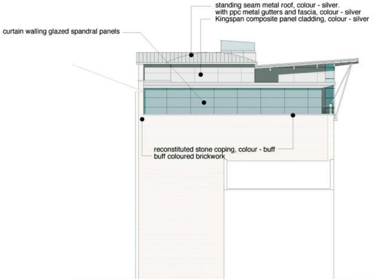
NORTH ELEVATION
